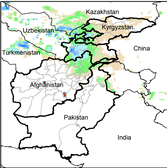
Daily Rainfall estimate for 30 Nov., 2014
