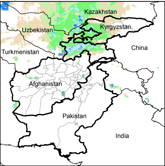
Daily Rainfall estimate for 6 Dec., 2014
