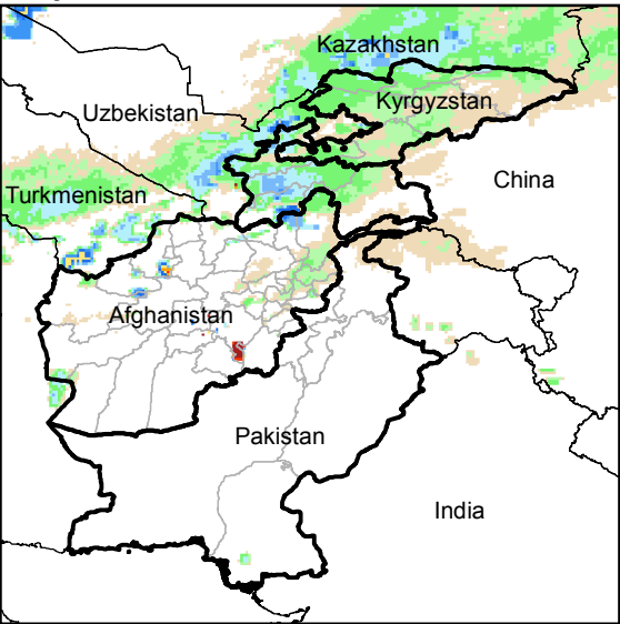
Daily Rainfall estimate for 7 Dec., 2014
