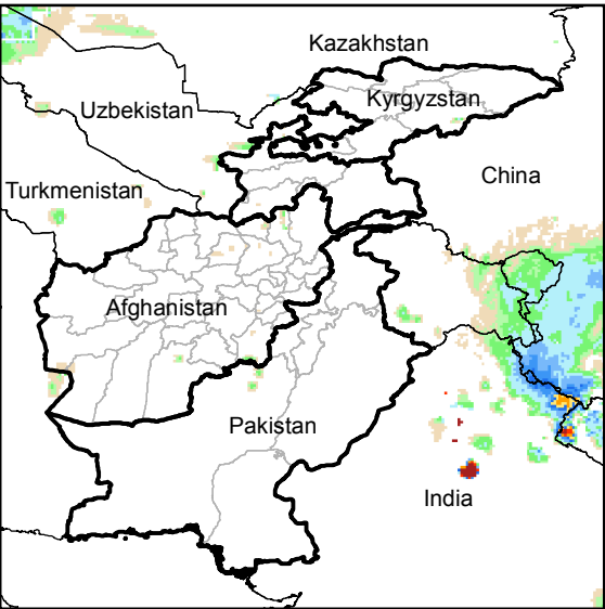
Daily Rainfall estimate for 18 Dec., 2014
