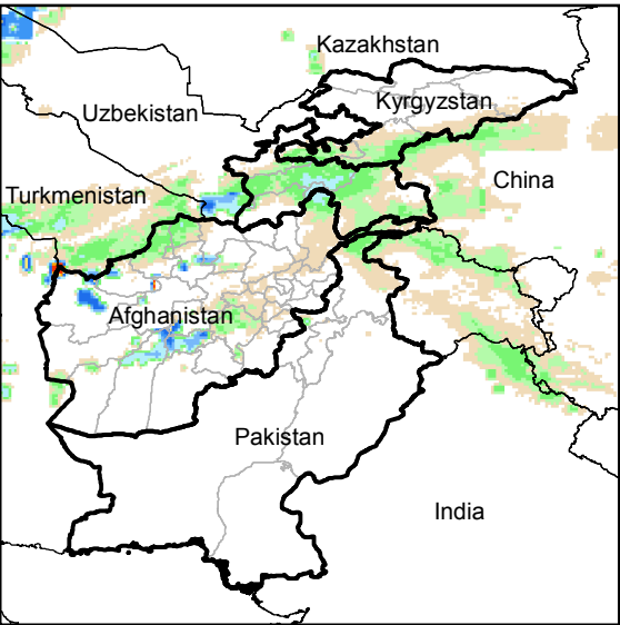
Daily Rainfall estimate for 25 Dec., 2014
