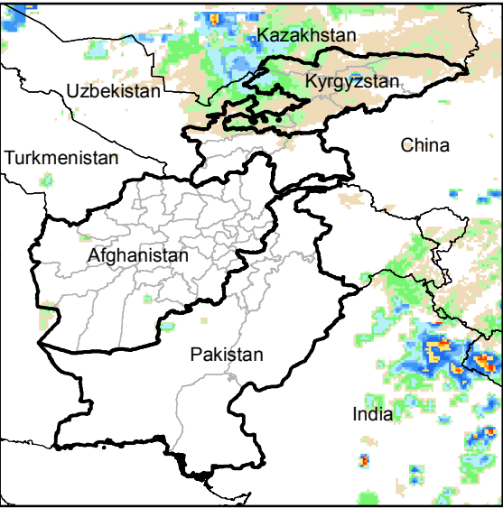
Daily Rainfall estimate for 2 Jan., 2015
