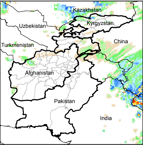
Daily Rainfall estimate for 3 Jan., 2015
