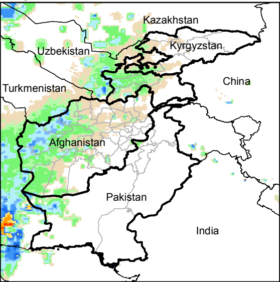
Daily Rainfall estimate for 22 Jan., 2015
