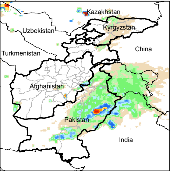
Daily Rainfall estimate for 2 Feb., 2015
