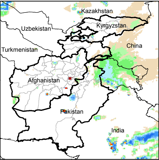
Daily Rainfall estimate for 8 Feb., 2015
