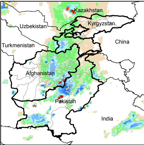
Daily Rainfall estimate for 10 Feb., 2015
