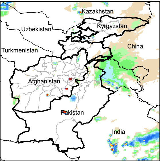
Daily Rainfall estimate for 11 Feb., 2015
