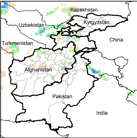
Daily Rainfall estimate for 17 Feb., 2015
