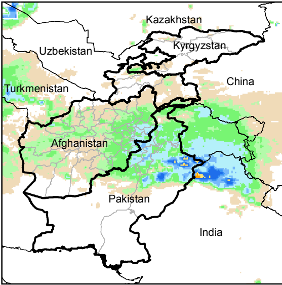
Daily Rainfall estimate for 20 Feb., 2015
