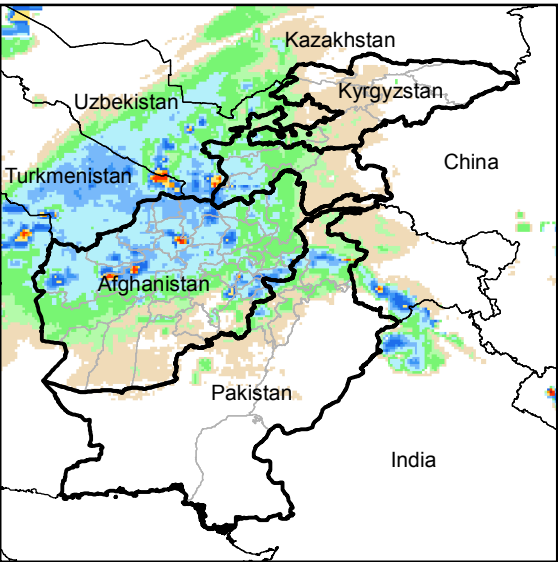
Daily Rainfall estimate for 18 Feb., 2015
