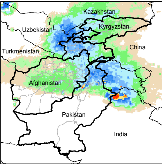
Daily Rainfall estimate for 19 Feb., 2015
