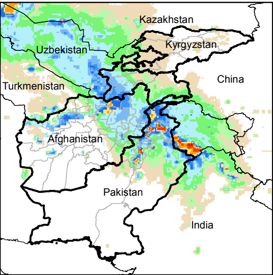
Daily Rainfall estimate for 27 Feb., 2015
