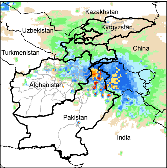
Daily Rainfall estimate for 28 Feb., 2015
