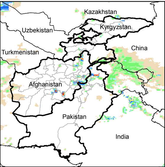
Daily Rainfall estimate for 20 Mar., 2015
