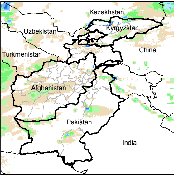
Daily Rainfall estimate for 21 Mar., 2015
