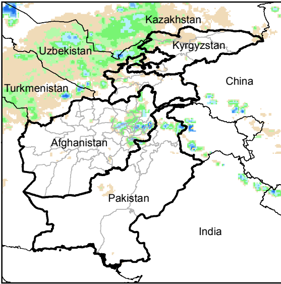
Daily Rainfall estimate for 22 Mar., 2015
