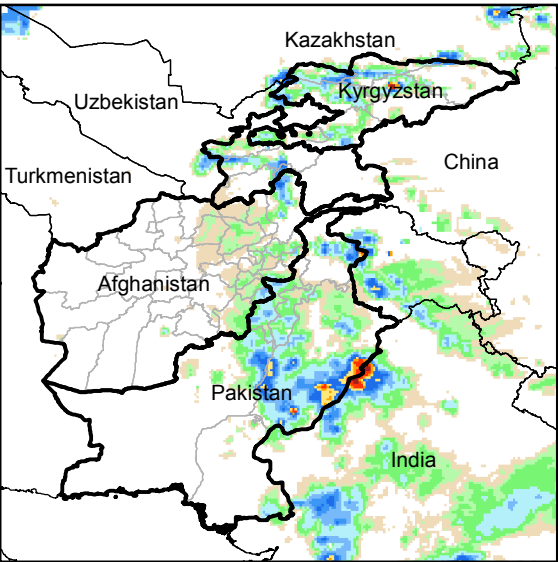
Daily Rainfall estimate for 14 Apr., 2015
