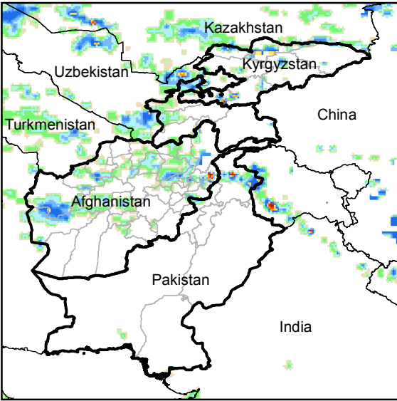
Daily Rainfall estimate for 17 Apr., 2015
