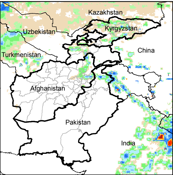
Daily Rainfall estimate for 16 Apr., 2015
