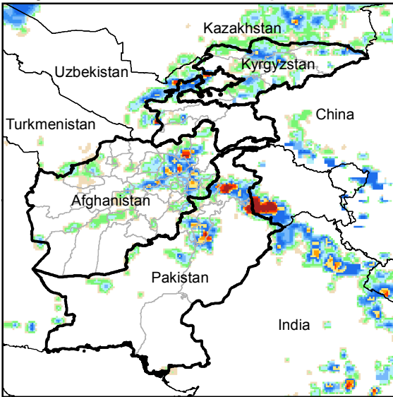
Daily Rainfall estimate for 18 Apr., 2015
