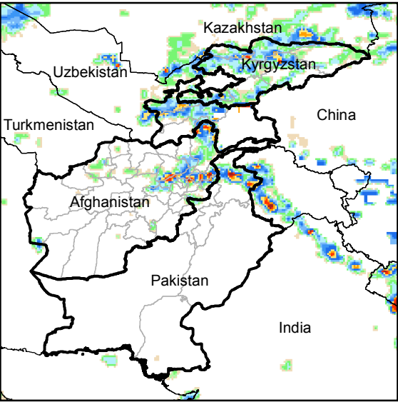
Daily Rainfall estimate for 24 Apr., 2015
