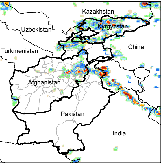
Daily Rainfall estimate for 25 Apr., 2015
