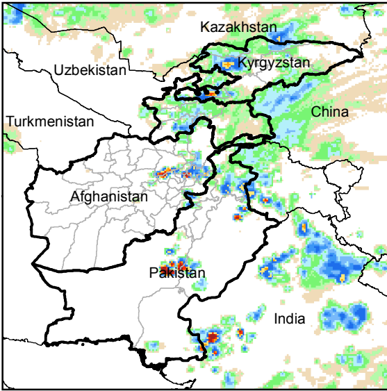
Daily Rainfall estimate for 13 May., 2015
