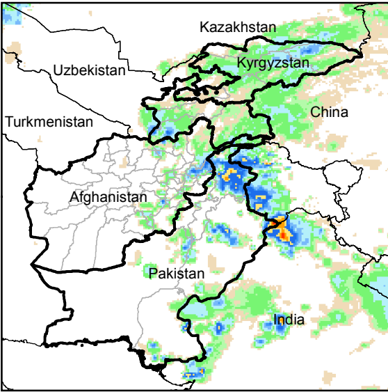
Daily Rainfall estimate for 12 May., 2015
