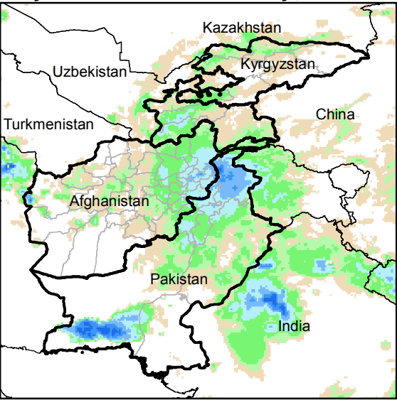
Daily Rainfall estimate for 11 May., 2015
