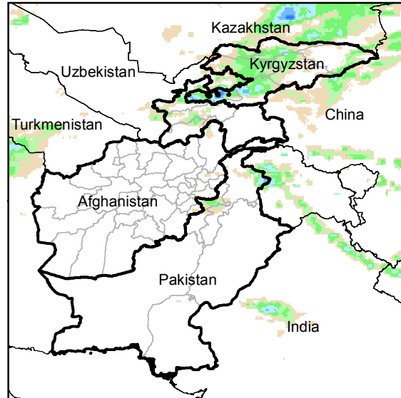
Daily Rainfall estimate for 21 May., 2015
