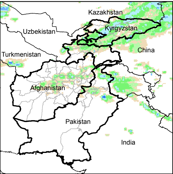
Daily Rainfall estimate for 25 May., 2015
