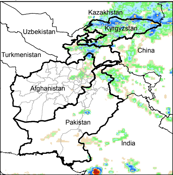
Daily Rainfall estimate for 12 Jun., 2015
