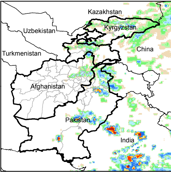
Daily Rainfall estimate for 15 Jun., 2015
