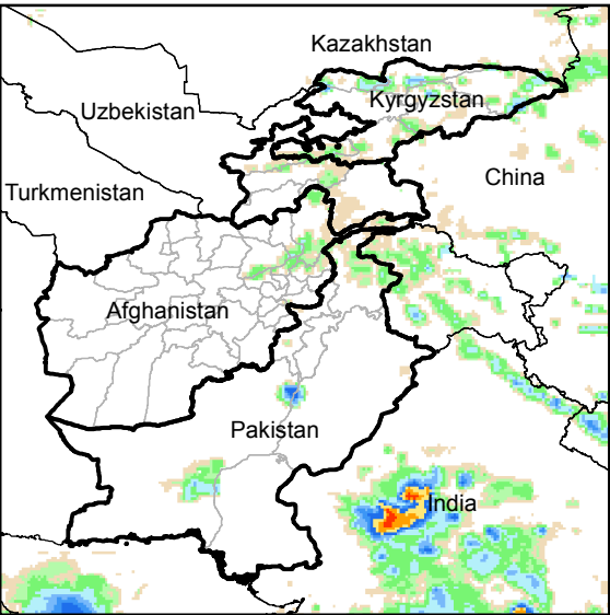
Daily Rainfall estimate for 14 Jun., 2015
