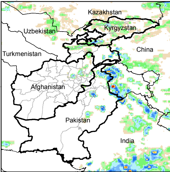
Daily Rainfall estimate for 16 Jun., 2015
