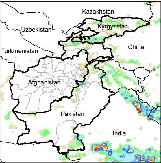
Daily Rainfall estimate for 22 Jun., 2015
