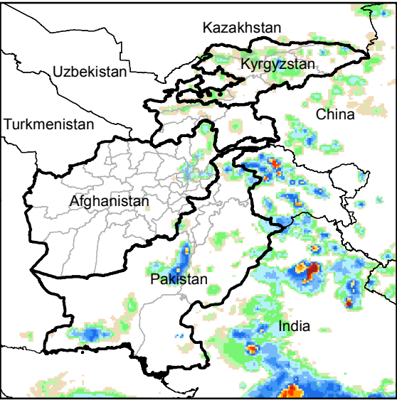
Daily Rainfall estimate for 21 Jun., 2015
