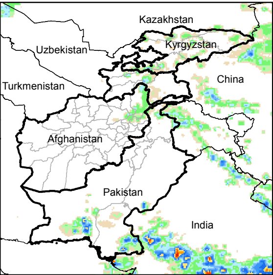
Daily Rainfall estimate for 20 Jun., 2015
