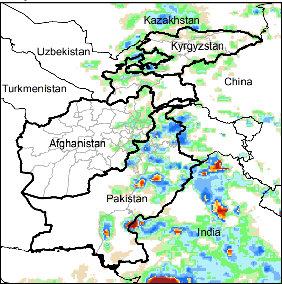
Daily Rainfall estimate for 26 Jun., 2015
