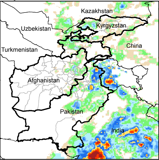
Daily Rainfall estimate for 24 Jun., 2015
