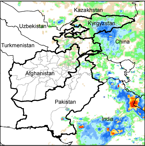
Daily Rainfall estimate for 25 Jun., 2015
