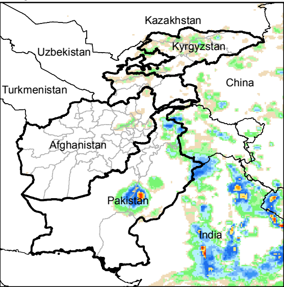
Daily Rainfall estimate for 2 Jul., 2015
