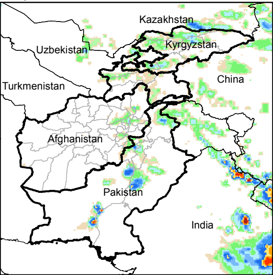
Daily Rainfall estimate for 1 Jul., 2015
