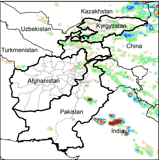
Daily Rainfall estimate for 30 Jun., 2015
