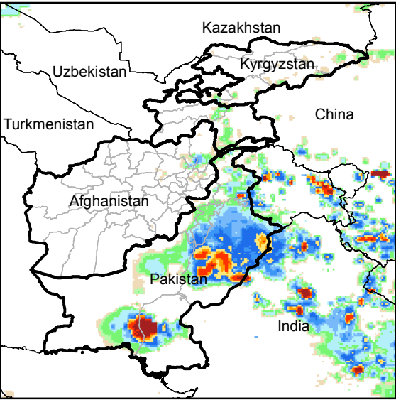
Daily Rainfall estimate for 7 Jul., 2015
