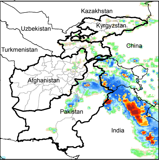
Daily Rainfall estimate for 6 Jul., 2015
