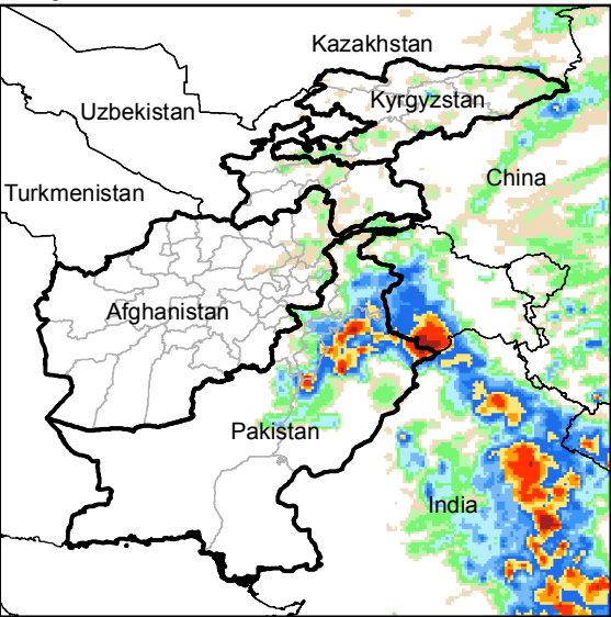
Daily Rainfall estimate for 13 Jul., 2015
