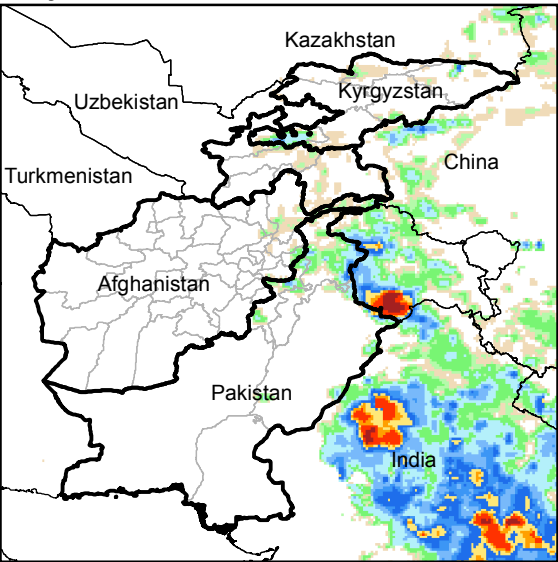
Daily Rainfall estimate for 12 Jul., 2015
