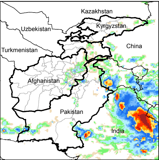
Daily Rainfall estimate for 15 Jul., 2015
