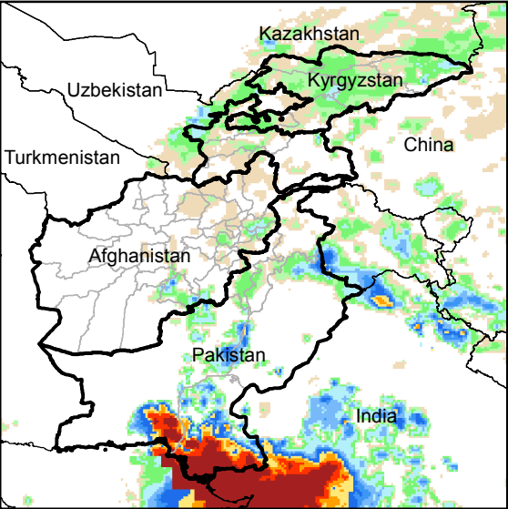
Daily Rainfall estimate for 28 Jul., 2015
