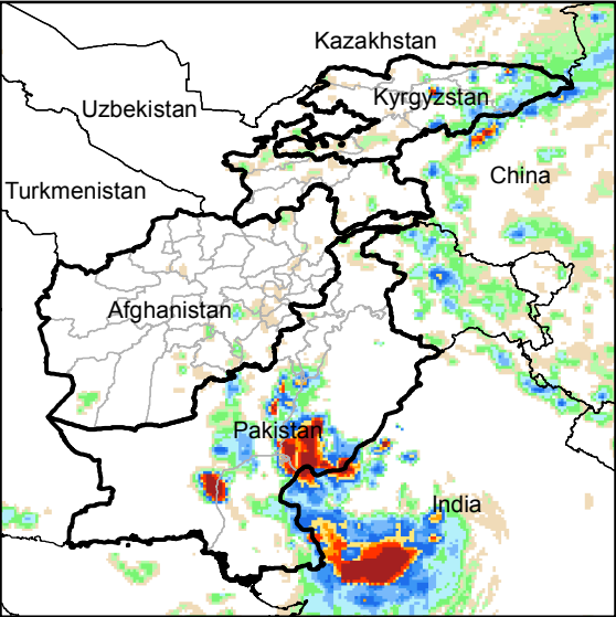
Daily Rainfall estimate for 29 Jul., 2015
