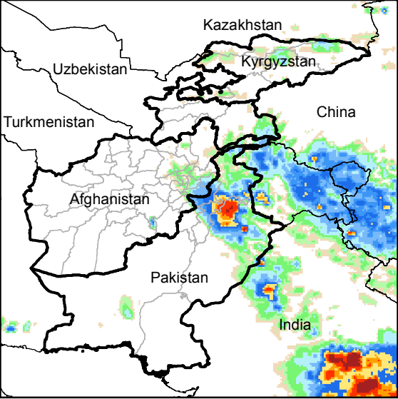
Daily Rainfall estimate for 3 Aug., 2015
