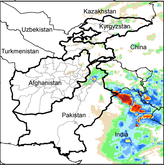
Daily Rainfall estimate for 8 Aug., 2015
