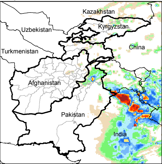
Daily Rainfall estimate for 11 Aug., 2015
