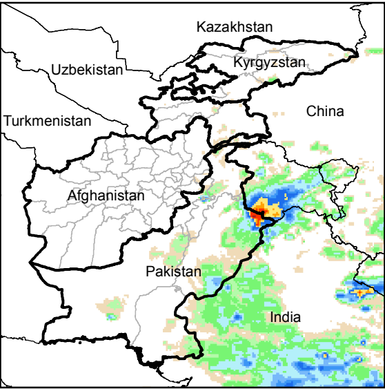
Daily Rainfall estimate for 12 Aug., 2015
