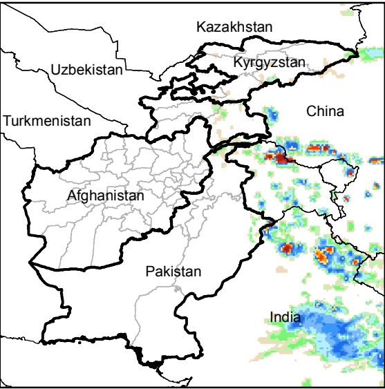
Daily Rainfall estimate for 19 Aug., 2015
