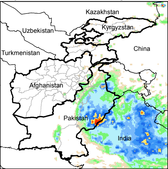
Daily Rainfall estimate for 18 Aug., 2015
