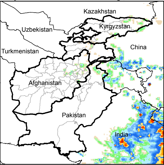
Daily Rainfall estimate for 17 Aug., 2015
