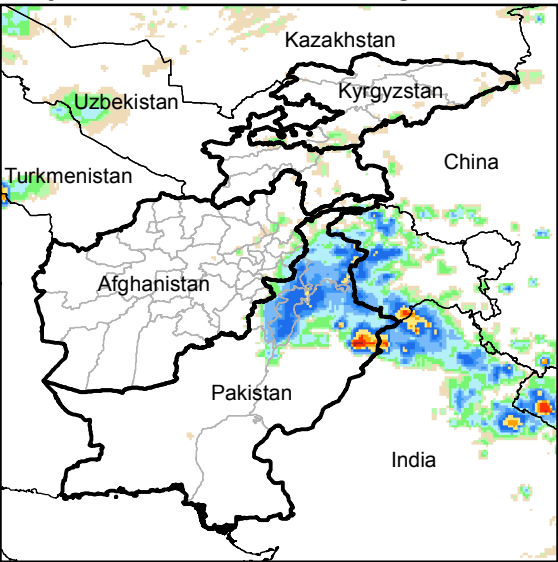
Daily Rainfall estimate for 24 Aug., 2015
