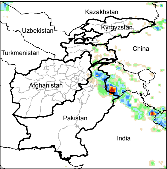
Daily Rainfall estimate for 23 Aug., 2015
