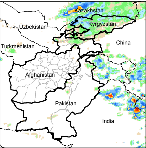
Daily Rainfall estimate for 25 Aug., 2015
