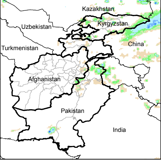
Daily Rainfall estimate for 5 Sep., 2015
