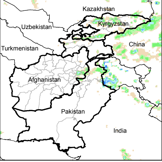
Daily Rainfall estimate for 6 Sep., 2015
