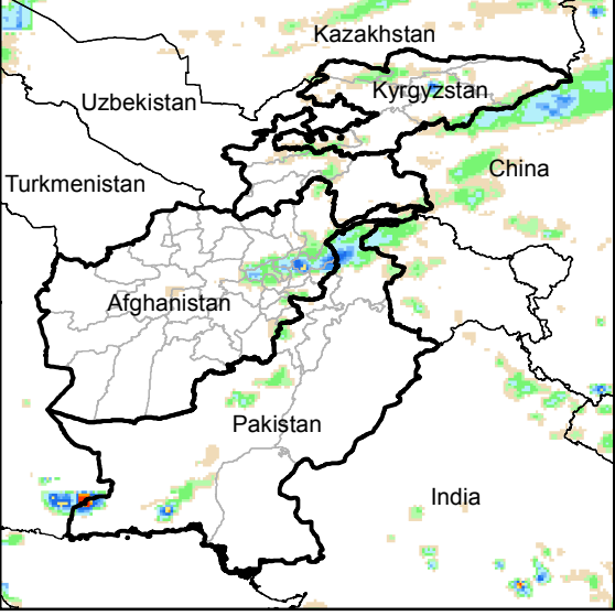
Daily Rainfall estimate for 4 Sep., 2015
