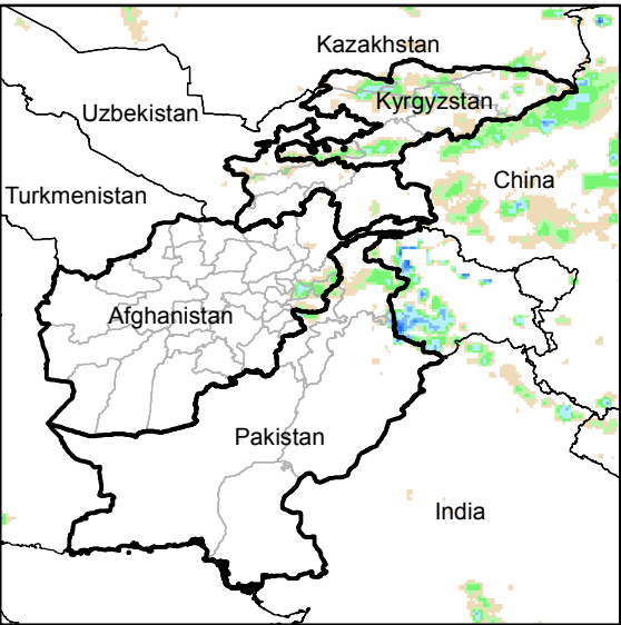
Daily Rainfall estimate for 9 Sep., 2015
