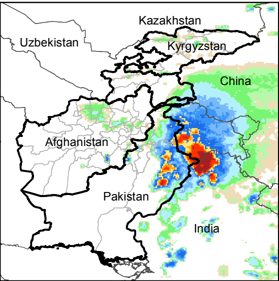
Daily Rainfall estimate for 25 Sep., 2015
