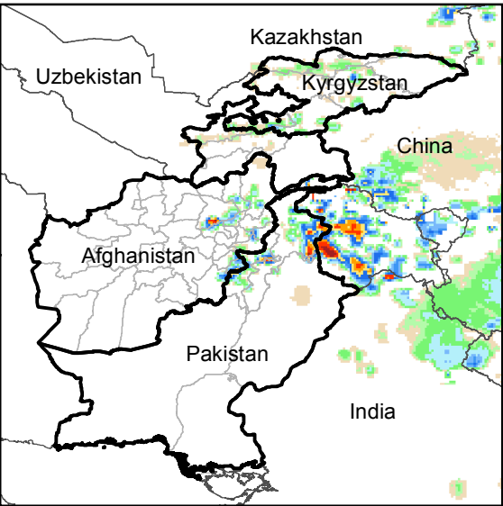
Daily Rainfall estimate for 26 Sep., 2015
