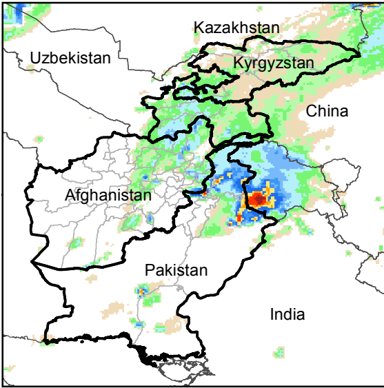
Daily Rainfall estimate for 19 Oct., 2015
