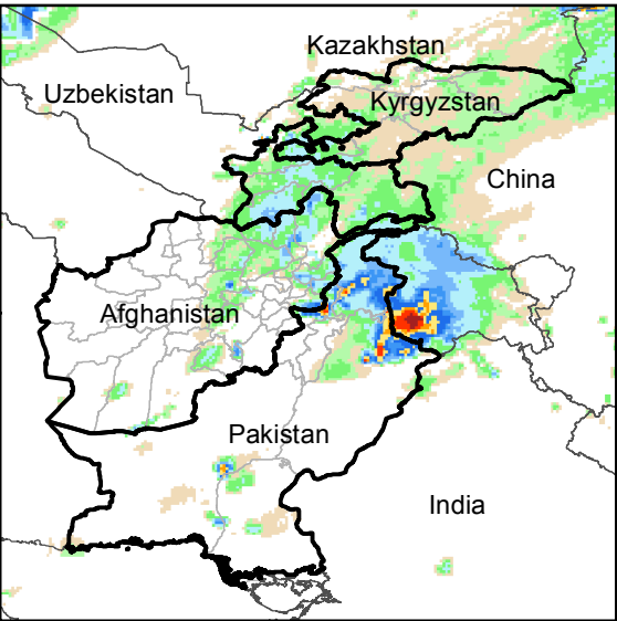
Daily Rainfall estimate for 22 Oct., 2015
