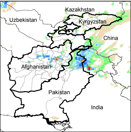
Daily Rainfall estimate for 23 Oct., 2015
