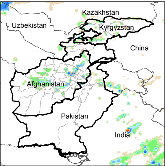
Daily Rainfall estimate for 27 Oct., 2015
