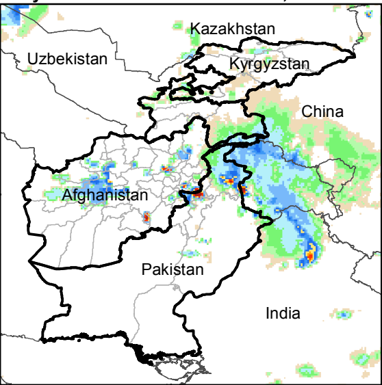
Daily Rainfall estimate for 26 Oct., 2015
