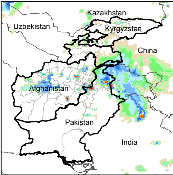
Daily Rainfall estimate for 29 Oct., 2015
