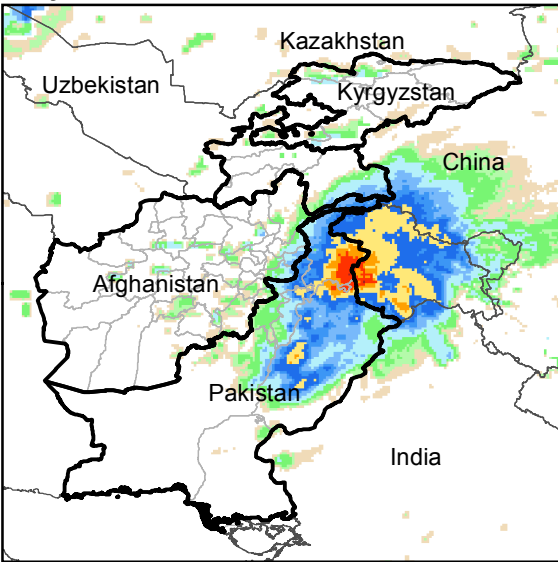
Daily Rainfall estimate for 28 Oct., 2015
