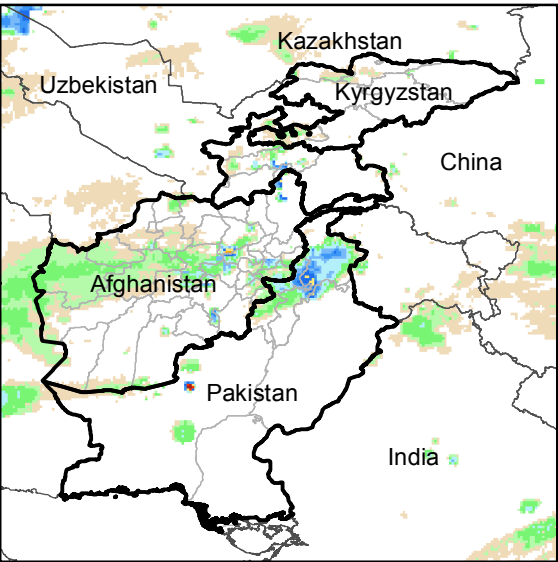
Daily Rainfall estimate for 13 Nov., 2015
