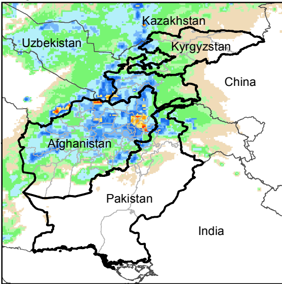
Daily Rainfall estimate for 15 Nov., 2015
