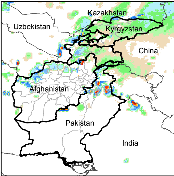
Daily Rainfall estimate for 13 Dec., 2015
