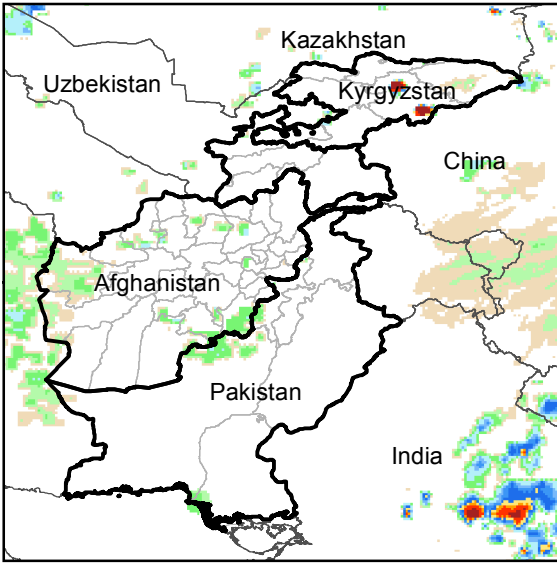
Daily Rainfall estimate for 19 Jan., 2016
