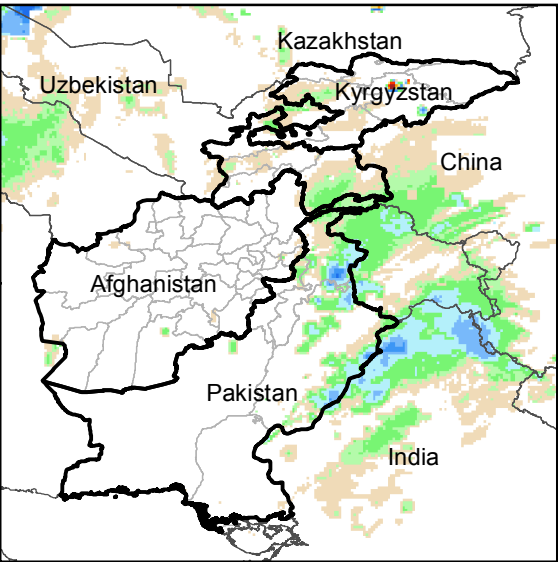
Daily Rainfall estimate for 22 Feb., 2016
