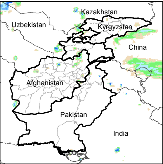
Daily Rainfall estimate for 25 Feb., 2016
